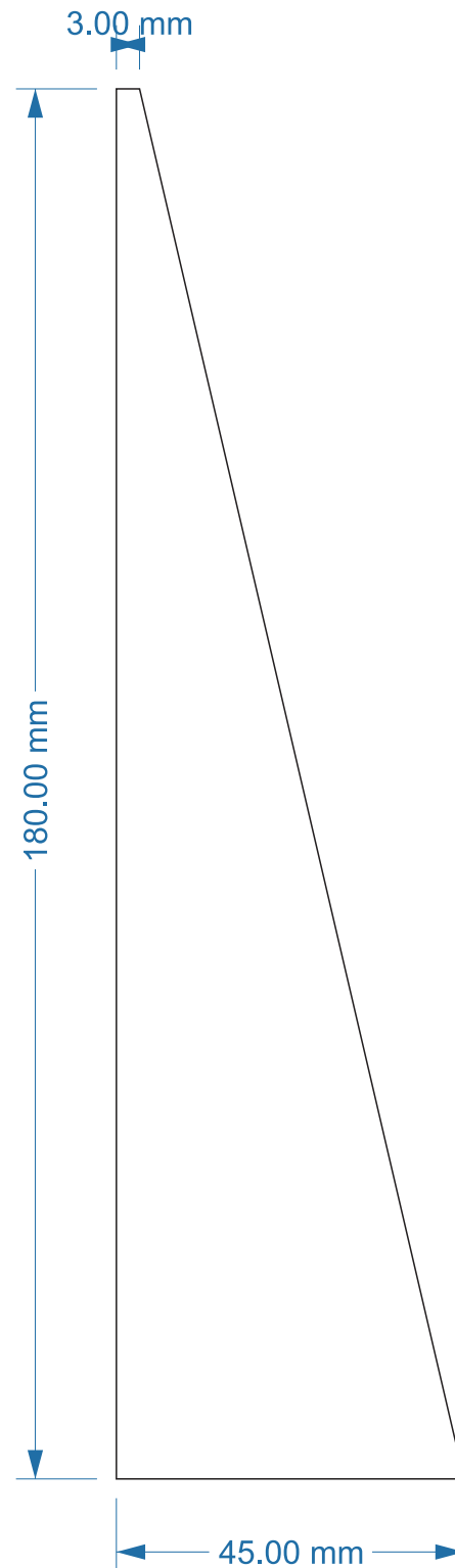
Side View
