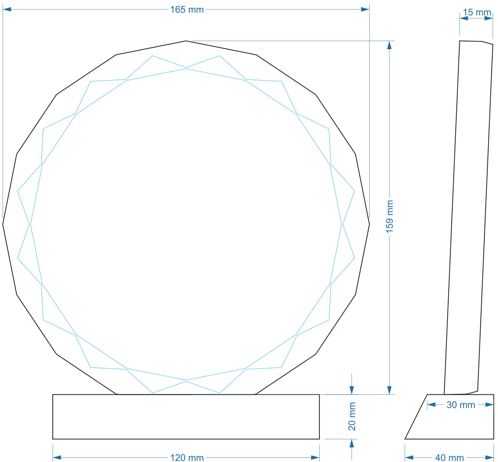
Front View
